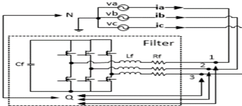
Figure 2: Modeling of Subsystem
