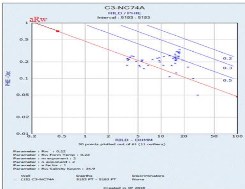
Fig. 8: Pickett plot result for unit D
