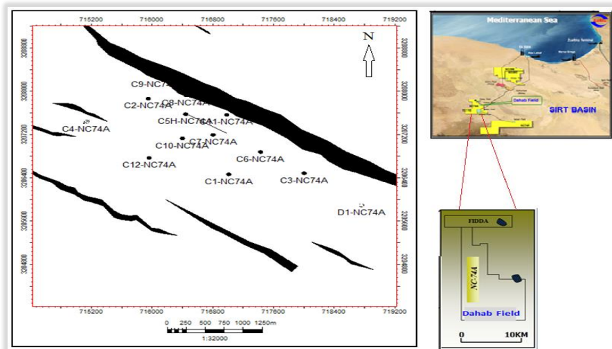
Fig.1: location map of study area, NC74A (Dahab Field) Sirt Basin. Basin, (Zueitina oil company2006).
