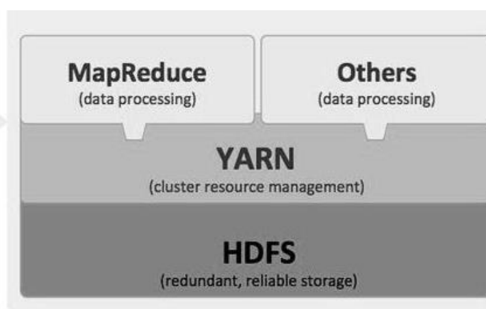
Figure 3: Hadoop Architecture.
