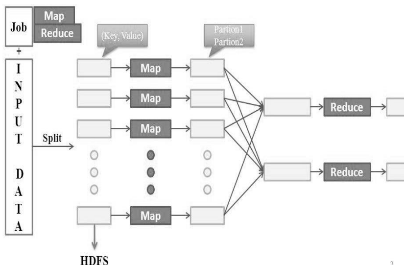
Figure 5: MapReduce Architecture
