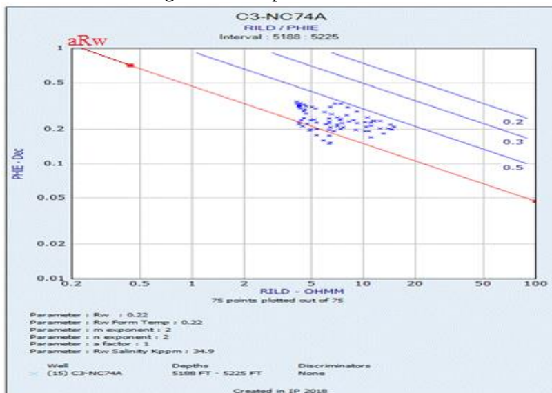
Fig. 8: Pickett plot result for unit D
