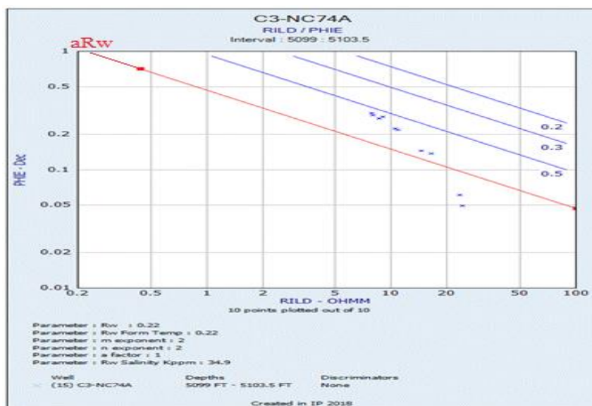
Fig. 5: Pickett plot result for unit A
